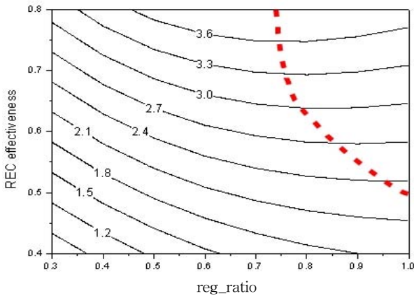
Fig. 4 Contour of cooling capacity of desiccant cooling system according to the area ratio of regeneration to dehumidification (rotation period of desiccant wheel = 180s).
