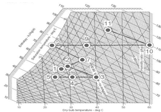
(b) Psychrometric chart
